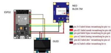
Gambar 7. Implementasi Hardware
