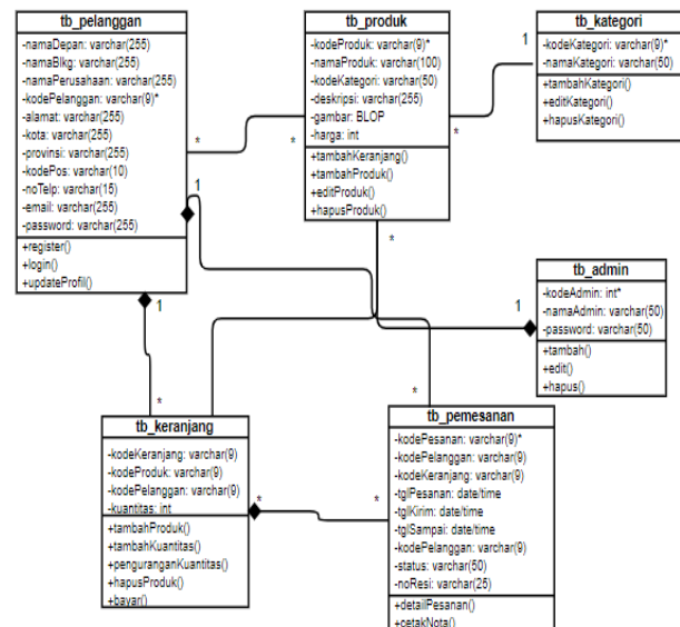
Gambar 2. Class Diagram
