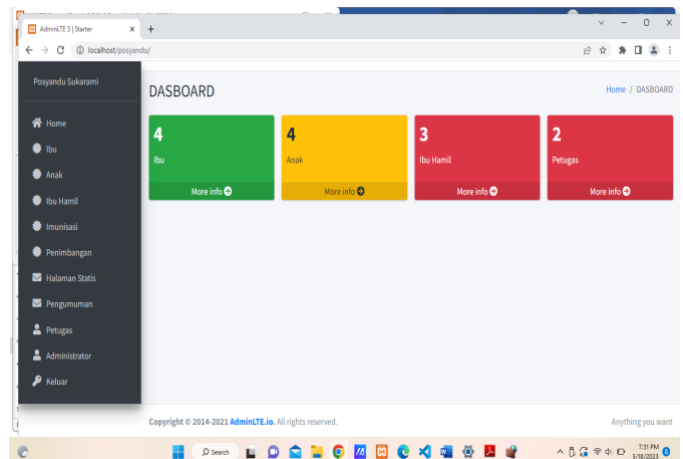
Gambar 2. Halaman Dashboard
