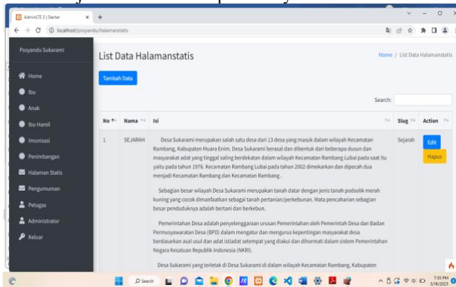
Gambar 8. Halaman Statis
