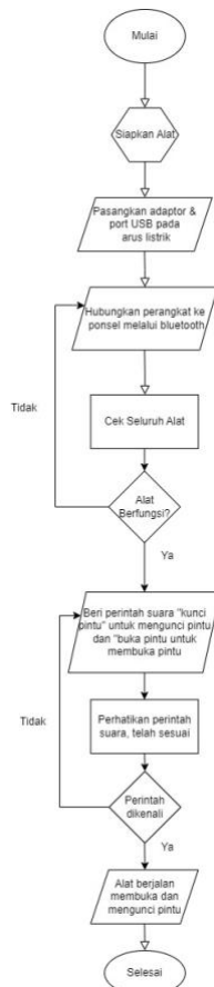
Gambar 4. Flowchart Sistem
