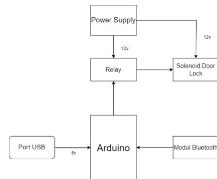
Gambar 3. Diagram Blok
