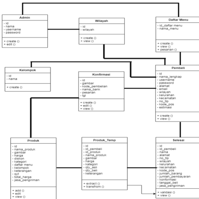
Gambar 6. Class Diagram
