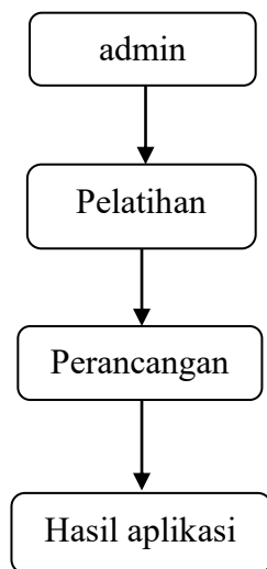
Gambar 1. Metode Penelitian
