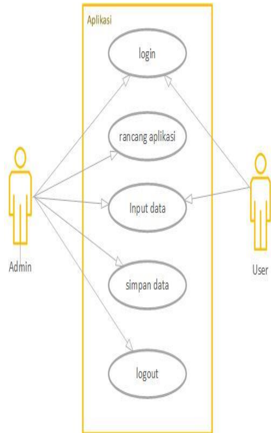
Gambar 2. Usecase diagram
