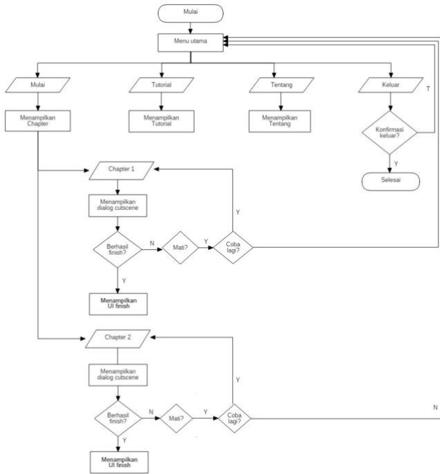
Gambar 2. Flowchart Game
