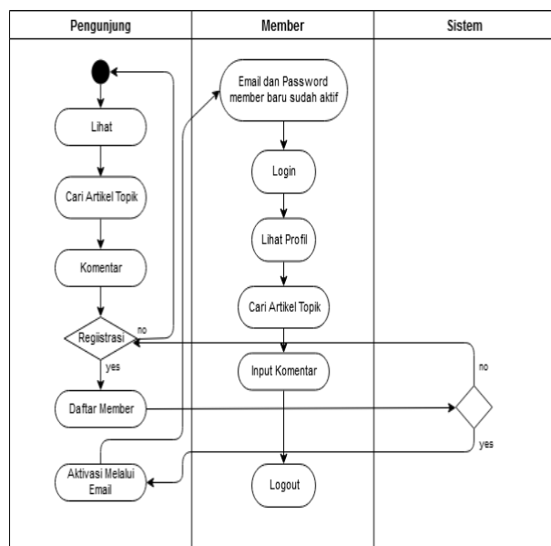
Gambar 3. Activity Diagram Sistem
