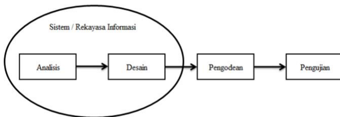
Gambar 1. Model Waterfall
